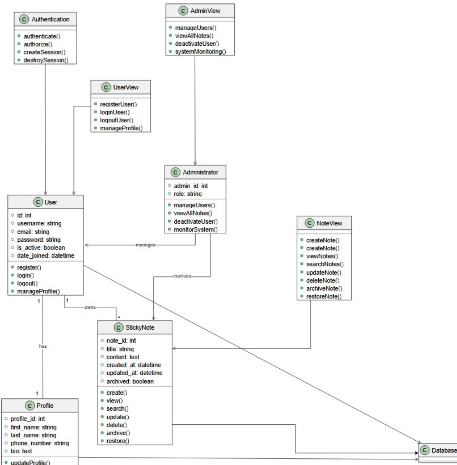
Sticky Notes System - Class Diagram
